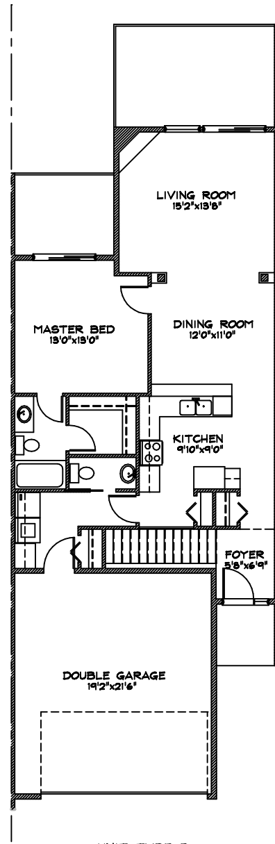
UNIT TYPE D GROUND FLOOR PLAN 1015 SQ.FT.
