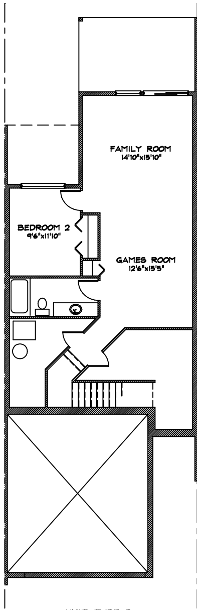
UNIT TYPE D BASEMENT FLOOR PLAN 705 SQ.FT.
