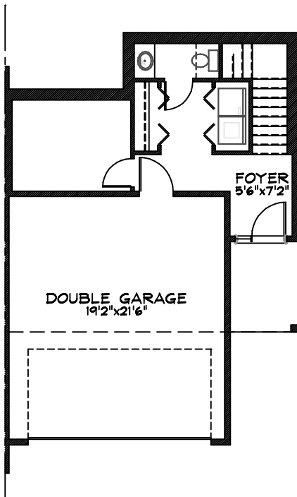
UNIT TYPE C BASEMENT FLOOR PLAN 140 SQ.FT.
