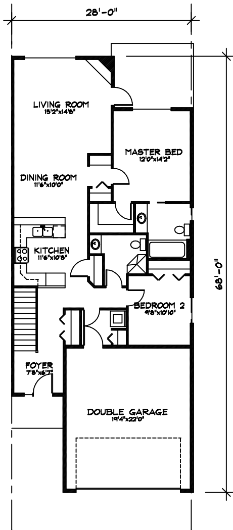
GROUND FLOOR PLAN 1229 SQ.FT. UNIT TYPE C
