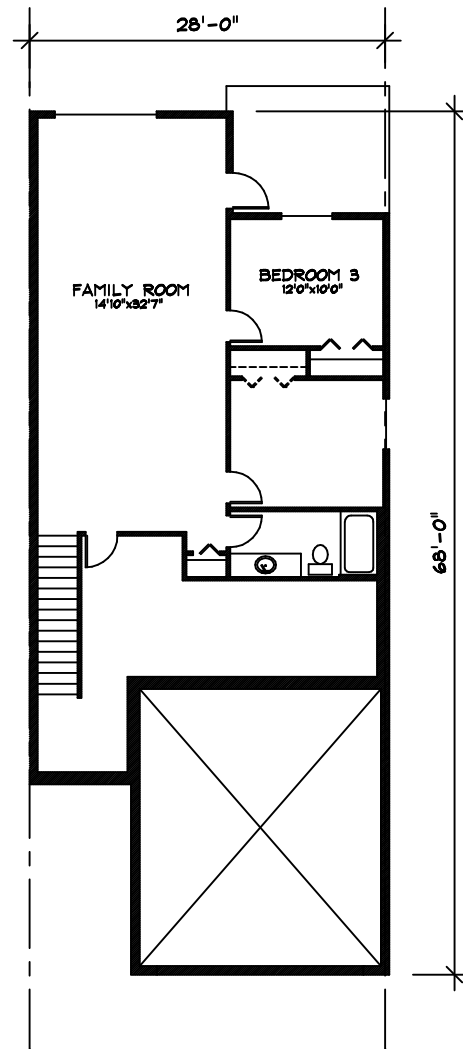
BASEMENT FLOOR PLAN 739 SQ.FT. UNIT TYPE C
