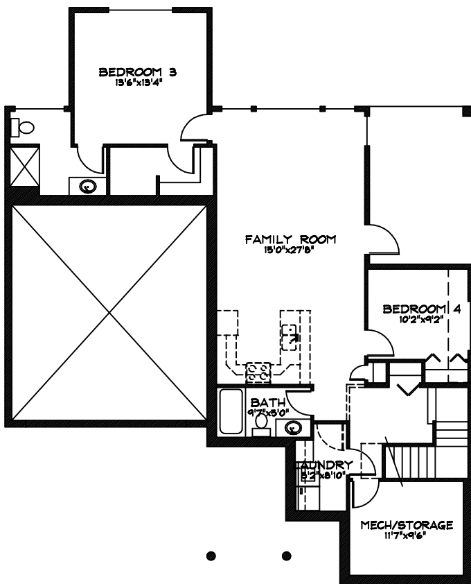
BASEMENT FLOOR PLAN 1116 SQ.FT.
