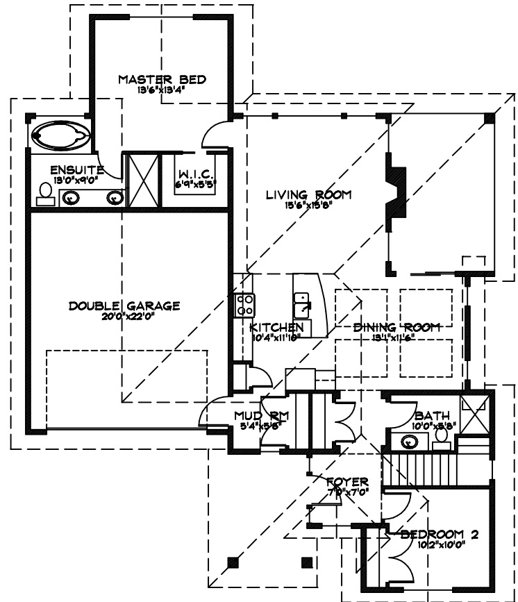
GROUND FLOOR PLAN 1293 SQ.FT.
