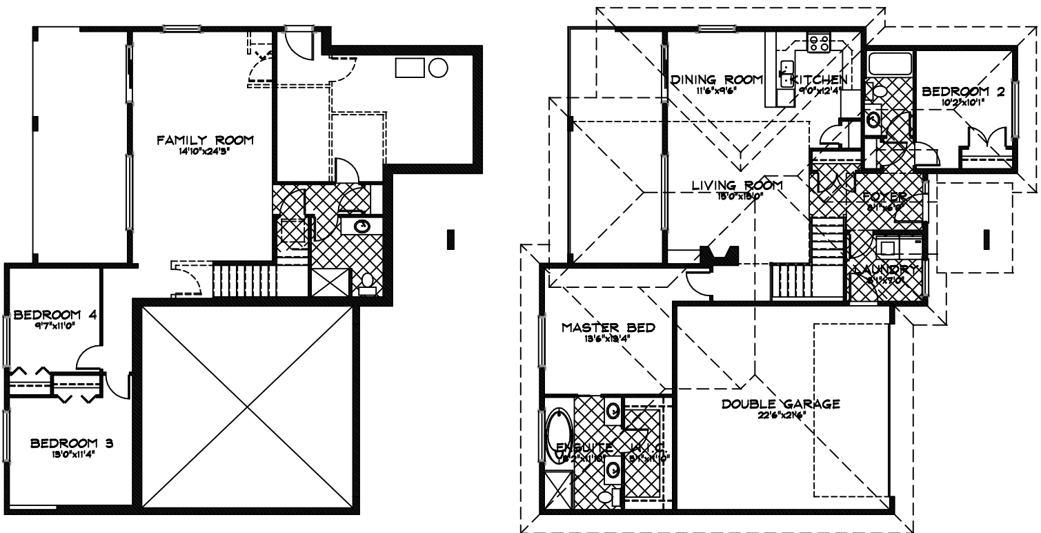
BASEMENT FLOOR PLAN 898 SQ.FT.
