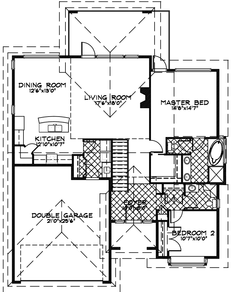
GROUND FLOOR PLAN 1525 SQ.FT.
